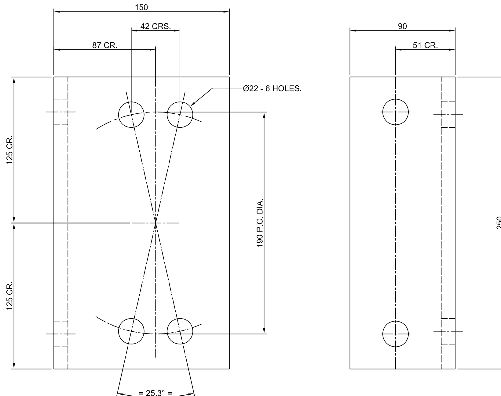
ITEM 9. 250 LONG x 150 x 90 x 12 THICK M.S. UNEQUAL ANGLE B.S. 4848: PART 4: 1972
